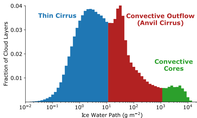
Figure 1. Histogram of the ice water path (IWP) of individual cloud layers with tops above 10 km in the tropical western Pacific (12°S to 12°N, 150–180°E). Three cloud types are identified for heuristic purposes using the histogram's two relative minima as boundaries. Layer IWP is calculated using the cloud retrievals described in section 2.1.1 prior correcting for the diurnal cycle of lidar sensitivity (see section 2.1.2). Bin widths are 0.1 in log space.
