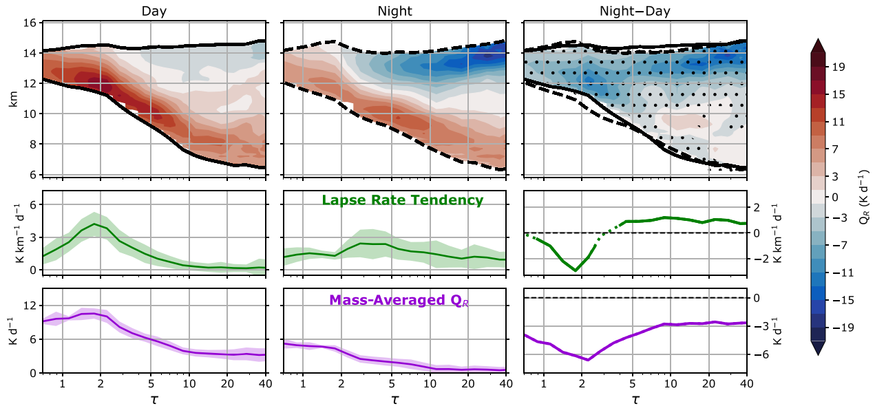
Figure 7. Net radiative heating rates for the (a) West Pacific and (b) Indian Ocean regions for (left) day, (middle) night, and (right) night minus day. For each region and time of day, the top plot shows the mean net heating rate of the 100-subsample composites. Stippling indicates a statistically significant diurnal difference ( \alpha = 0.01 ), and black lines (solid for day and dashed for night) show median CTH and CBH. The middle and bottom rows show the 100-subsample mean lapse rate tendency (LRT) and mass-averaged layer heating ( \bar{Q}_R ), respectively. Shading indicates the standard deviation of the subsample composites. The lines showing night-day LRT are solid where the difference is statistically significant and dotted otherwise. The night-day \bar{Q}_R is statistically significant at all \tau .
